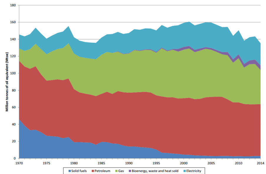
Chart 3 Final energy consumption by fuel, UK (1970 to 2014)
